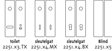
blind 2251.X0 cilinder 2251.X2.RX cilinder 2251.X2.EX cilinder 2251.X2.KX cilinder 2251.X2.UX
