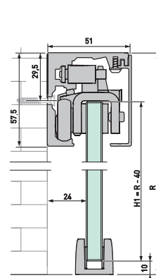
Portavant 60 Montage mural
