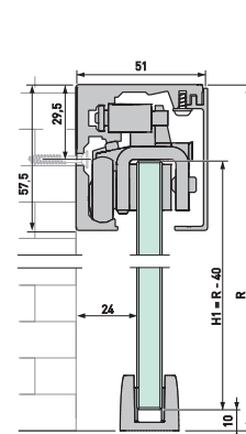
Portavant 60 Wandmontage
