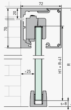
Two-sash systems without sidelight
