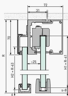
One-sash systems without sidelight
