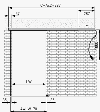
One-sash systems without sidelight
