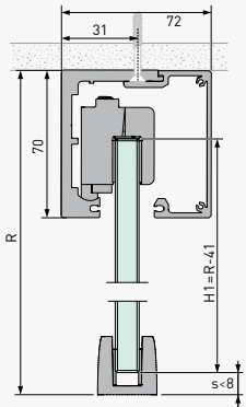
One-sash systems without sidelight
