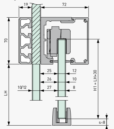
Track mounted on glass façade
