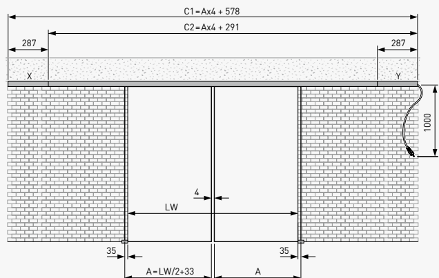
Two-sash systems without sidelight
